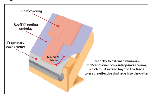
Figure 2 - Eaves Detail
